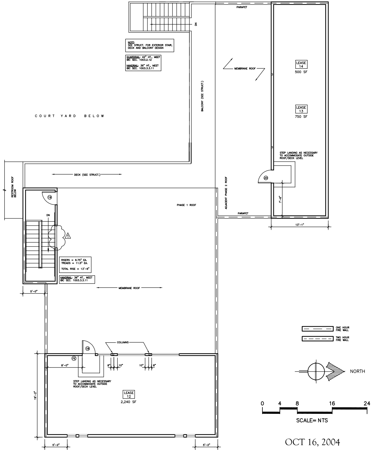
2nd Floor Plan - Phases 1, 2 & 3
